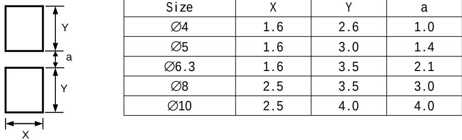
Recommended Land Size (Unit: mm)
