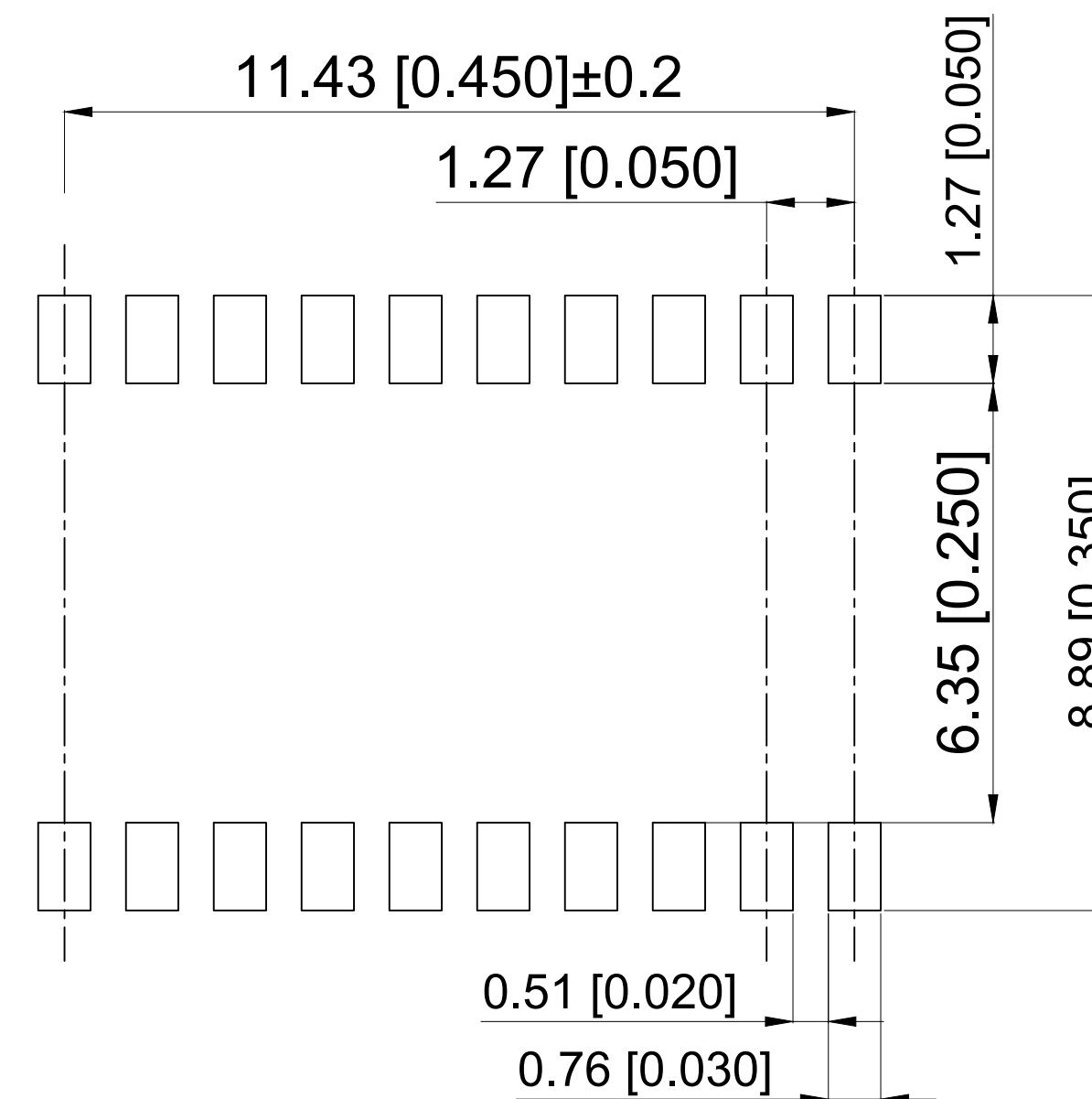
PCB LAYOUT
