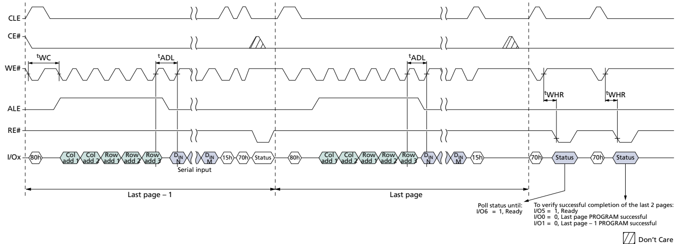
Figure 88: PROGRAM PAGE CACHE Ending on 15h
