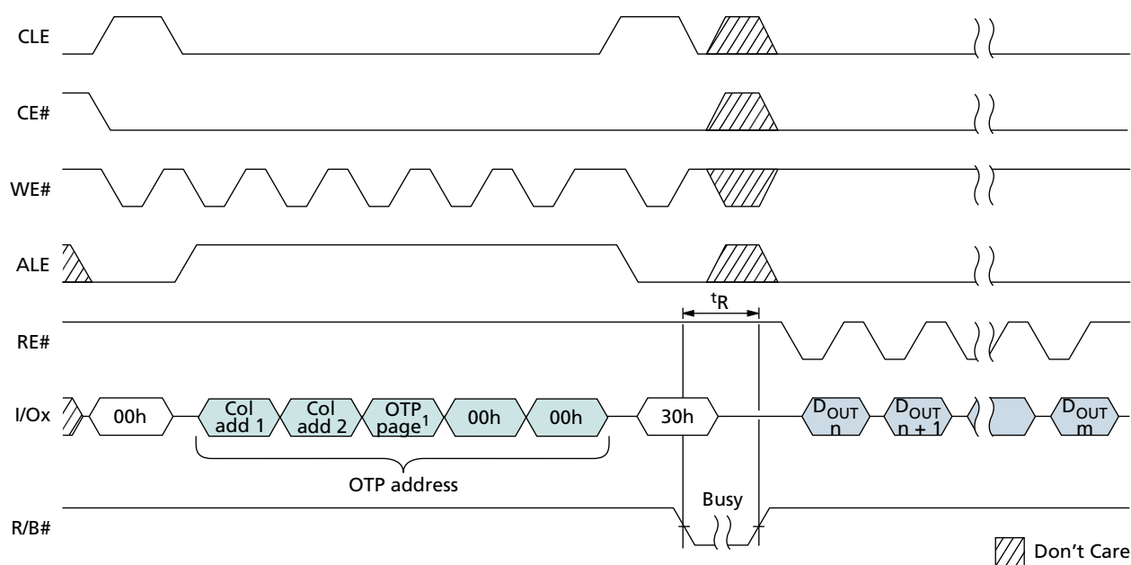
Figure 62: OTP DATA READ
