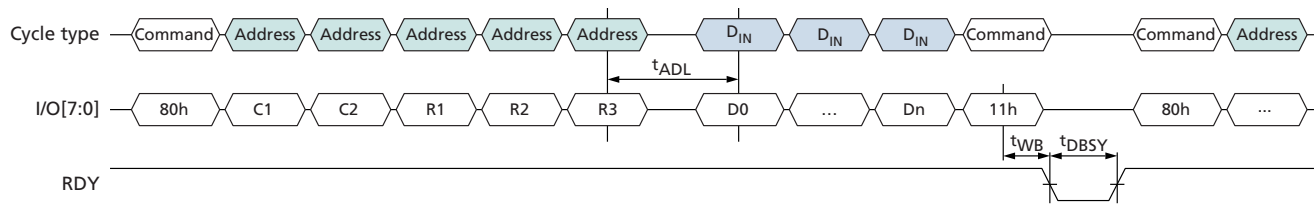
Figure 43: PROGRAM PAGE TWO-PLANE (80h–11h) Operation
