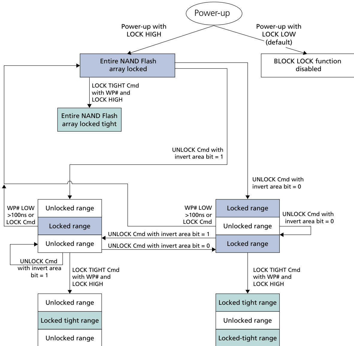
Figure 58: BLOCK LOCK Flowchart
