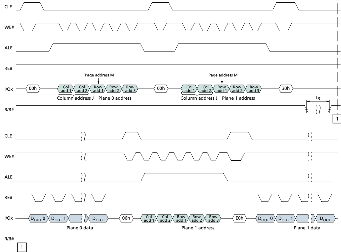
Figure 39: READ PAGE TWO-PLANE (00h-00h-30h) Operation
