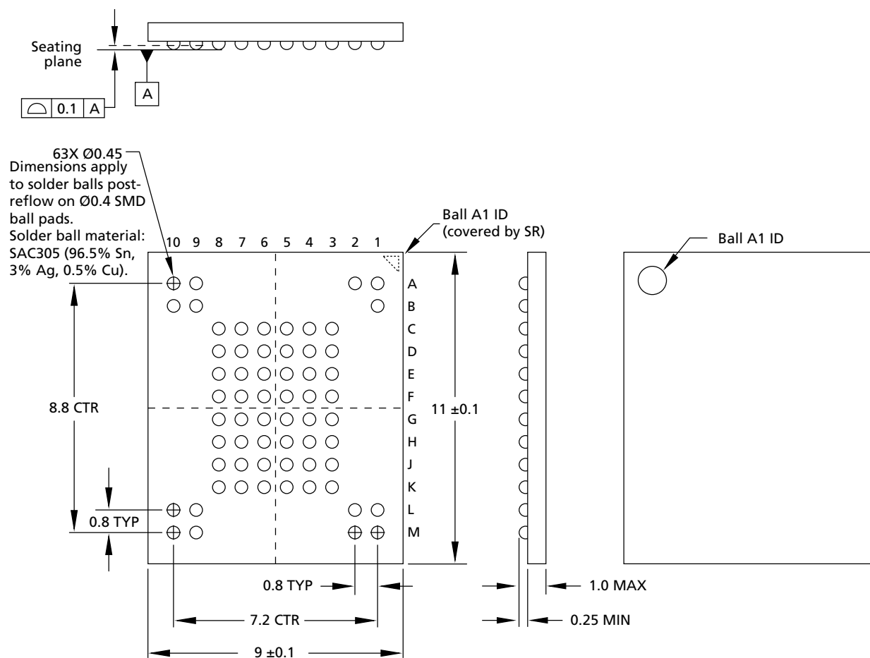
Figure 6: 63-Ball VFBGA
