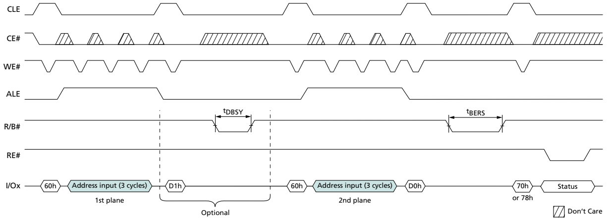
Figure 73: TWO-PLANE/MULTIPLE-DIE READ STATUS Cycle
