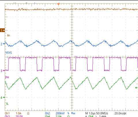
CH1: Input current, 1A/div; CH2: system voltage AC), 200mV/div, CH3: PHASE, 20V/div, CH4: (inductor current, 2A/div, 1μs/div
