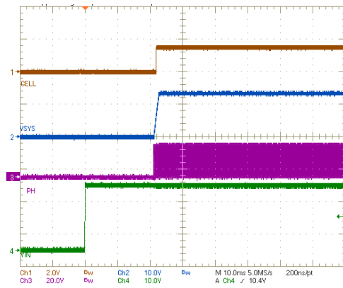
CH1: CELL, 2V/div, CH2: SRN, 10V/div, CH3: PHASE, 20V/div, CH4: VCC, 10V/div, 10ms/div
