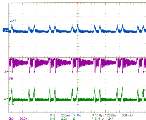
CH2: system voltage (AC), 200mA/div, CH3: PHASE, 20V/div, CH4: inductor current, 2A/div, 10μs/div
