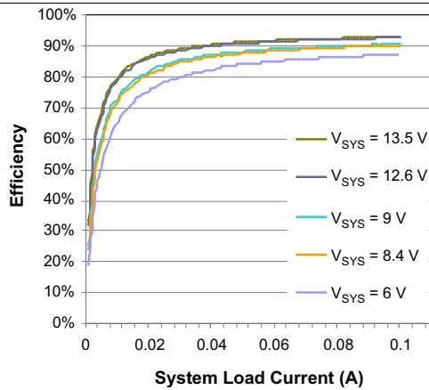
Figure 4. Light Load Efficiency vs. System Current
