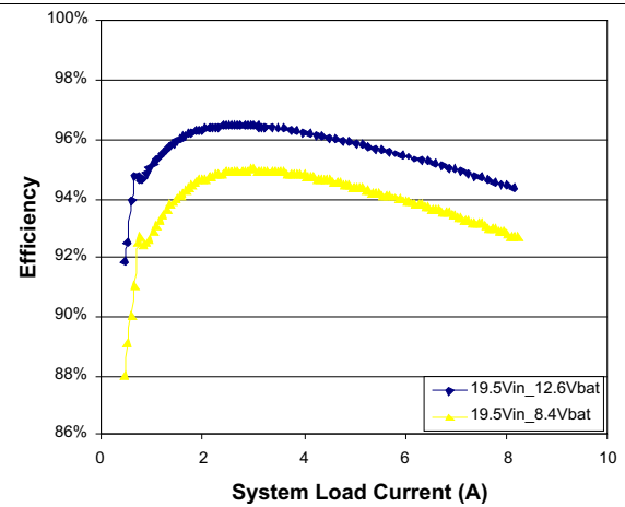
Figure 5. Heavy Load Efficiency vs. System Current
