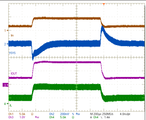
CH1: Input current, 2A/div; CH2: system voltage(AC), 200mv/div; CH3: IOUT, 1V/div; CH4: inductor current, 2A/div, 200μs/div
