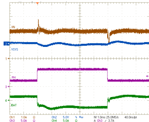
CH1: input current, 1A/div; CH2: system voltage (AC), 5V/div; CH3: system load, 5A/div; CH4: battery charge current, 5A/div, 1ms/div Figure 19. 2 to 6 A System Load Transient (IDPM Enable and Charge Enable)
