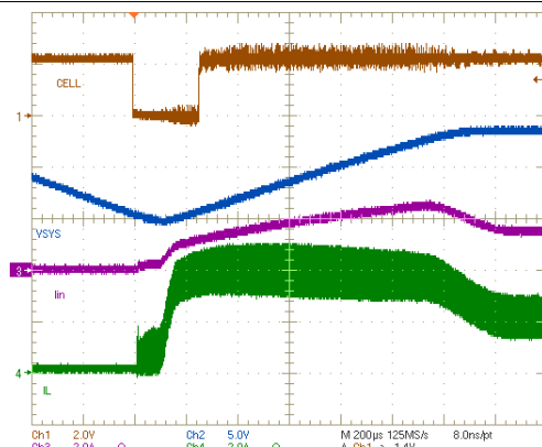
CH1: CELL, 2V/div, CH2: system voltage, CH3: input current, 2A/div, 5V/div, CH4: inductor current, 2A/div, 200μs/div
