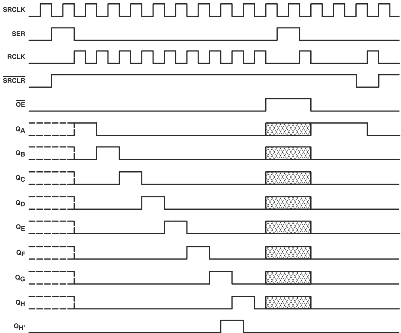
Figure 6-1. Timing Diagram
