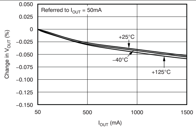
Figure 2. Load Regulation
