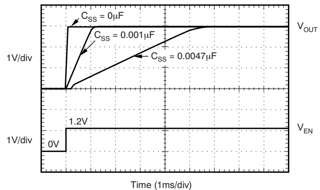
Figure 31. Turnon Response
