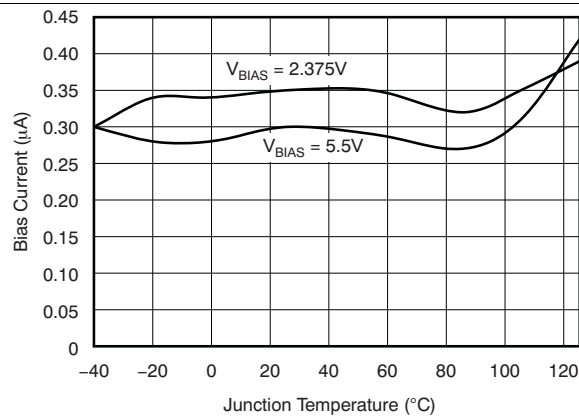
Figure 15. I_{BIAS} Shutdown vs Temperature
