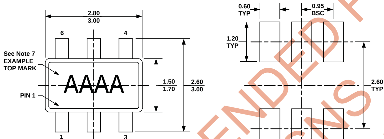
TOP VIEW
