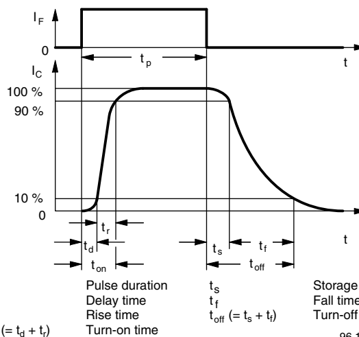
Fig. 4 - Switching Times
