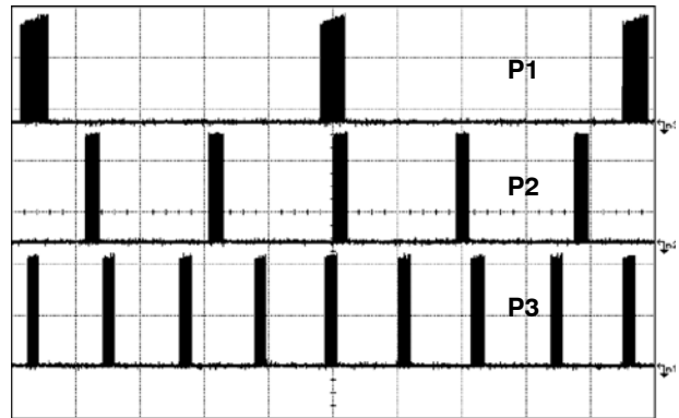
Figure 18. Output pulses at various power levels ( X = 5\text{ }\mu\text{s/div} ) P1 < P2 < P3
