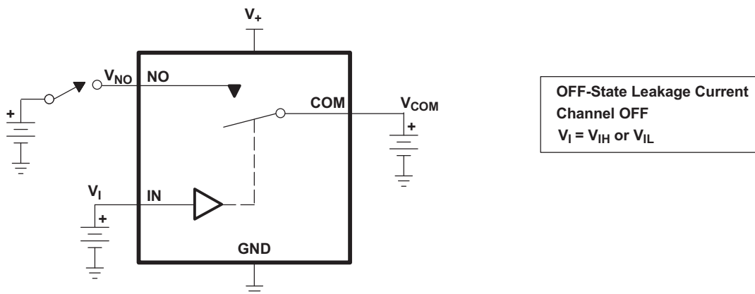
Figure 12. OFF-State Leakage Current ( I_{COM(OFF)} , I_{NC(OFF)} , I_{COM(PWROFF)} , I_{NC(PWRFF)} )
