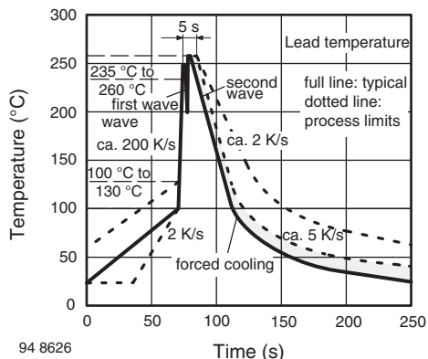
Fig. 18 - Wave Soldering Double Wave Profile According to J-STD-020 for DIP-8 Devices
