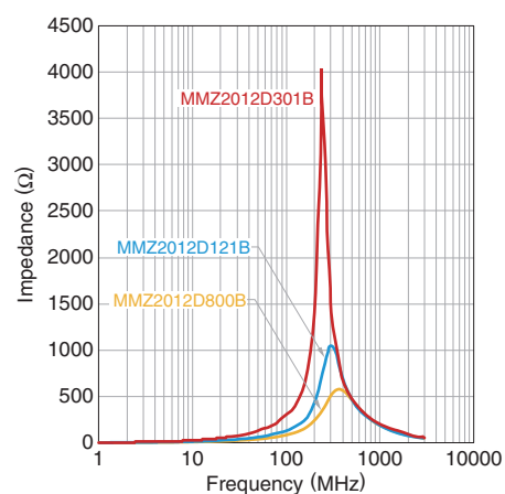
MMZ2012D series
