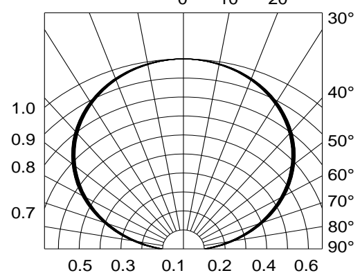
Fig.6-Radiation Diagram
