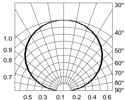
Fig.6-Radiation Diagram Ta=25°C
