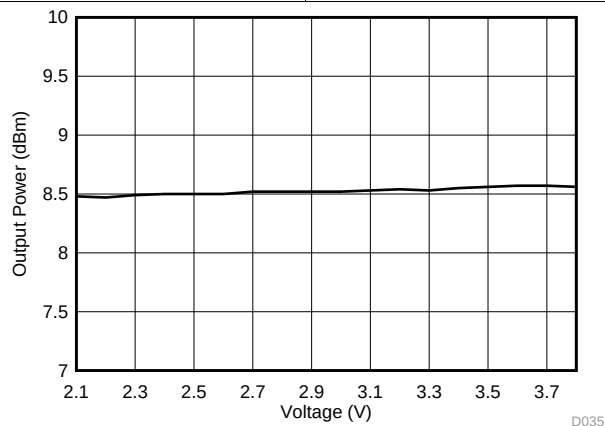
Figure 5-45. TX Bluetooth low energy Maximum Output Power vs VDD, 2440 MHz
