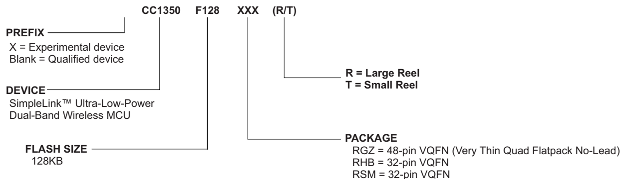
Figure 8-1. Device Nomenclature
