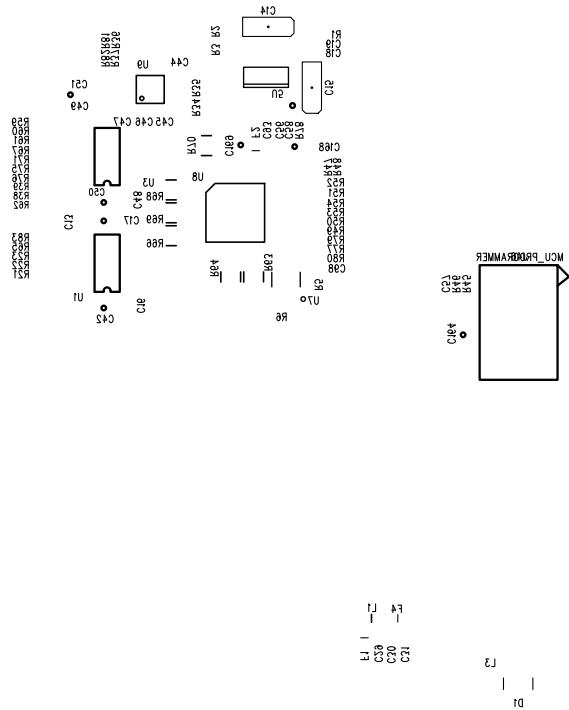
Figure 51. Quark Baseboard Bottom Silkscreen
