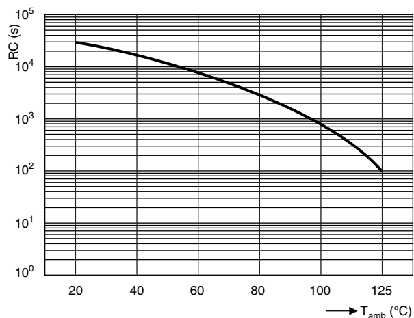
Insulation resistance as a function of temperature R_{1s} = f(T_A), T_{LL} \leq T_A \leq T_{UL}
