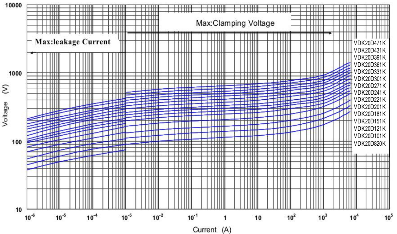
V-I Curve (VDK-20D820K to VDK-20D471K)
