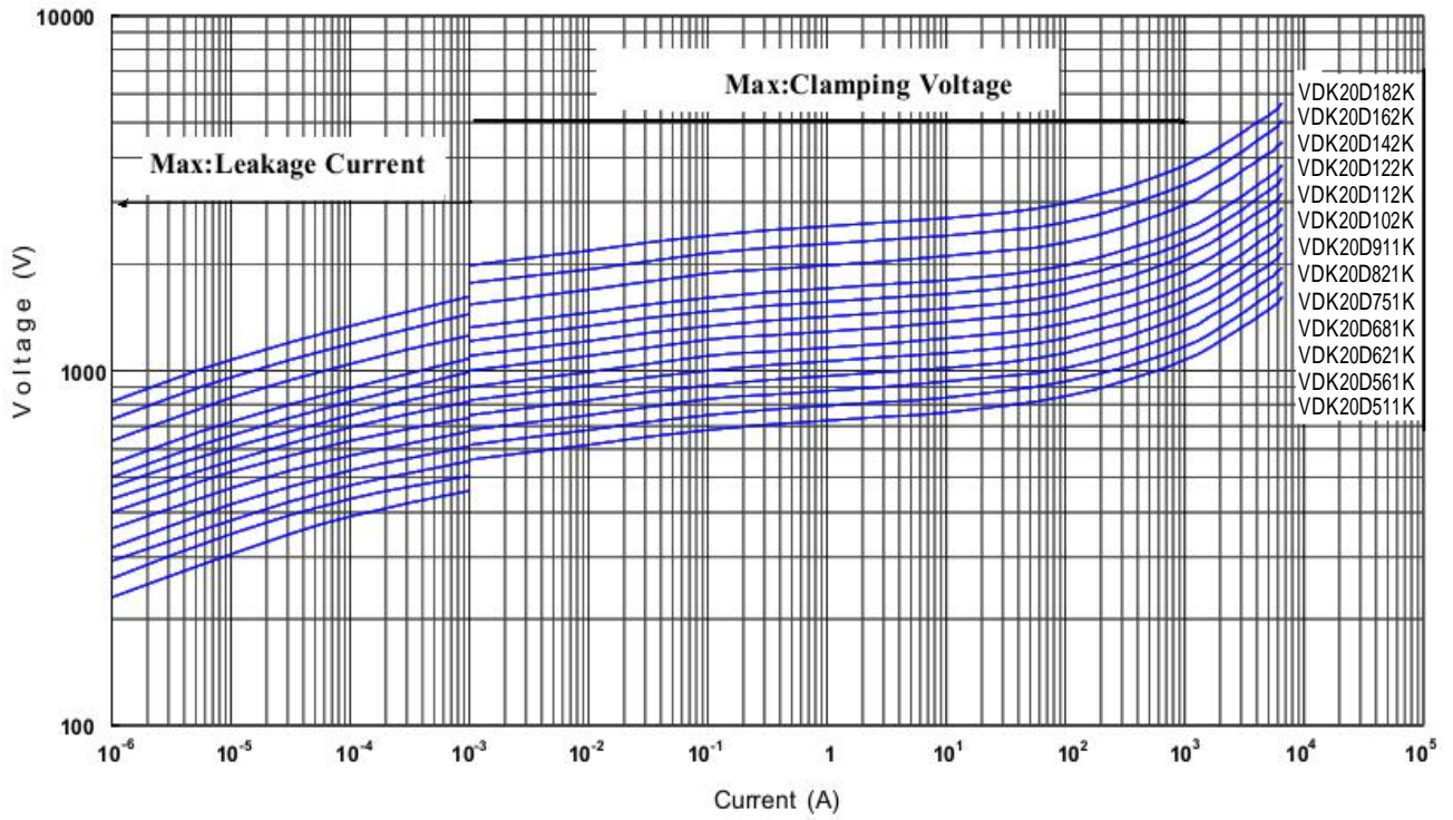
V-I Curve (VDK-20D511K to VDK-20D182K)
