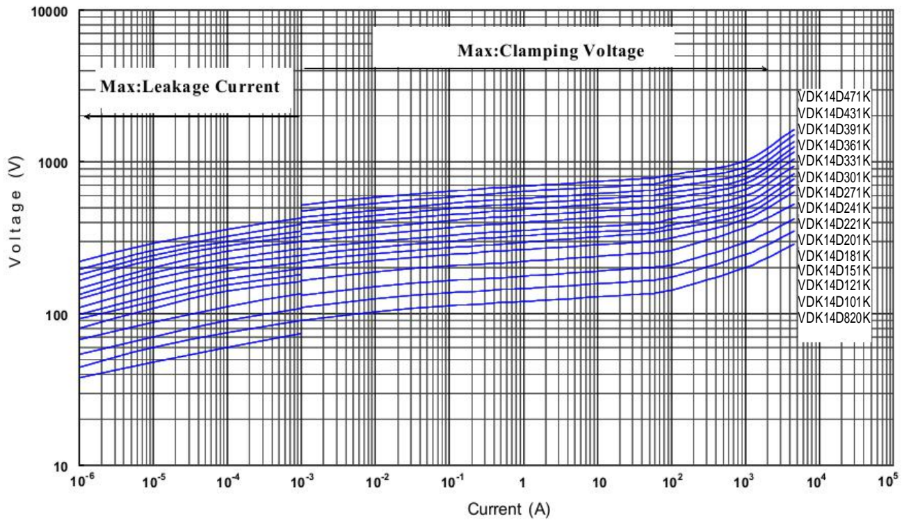
V-I Curve (VDK-14D820K to VDK-14D471K)
