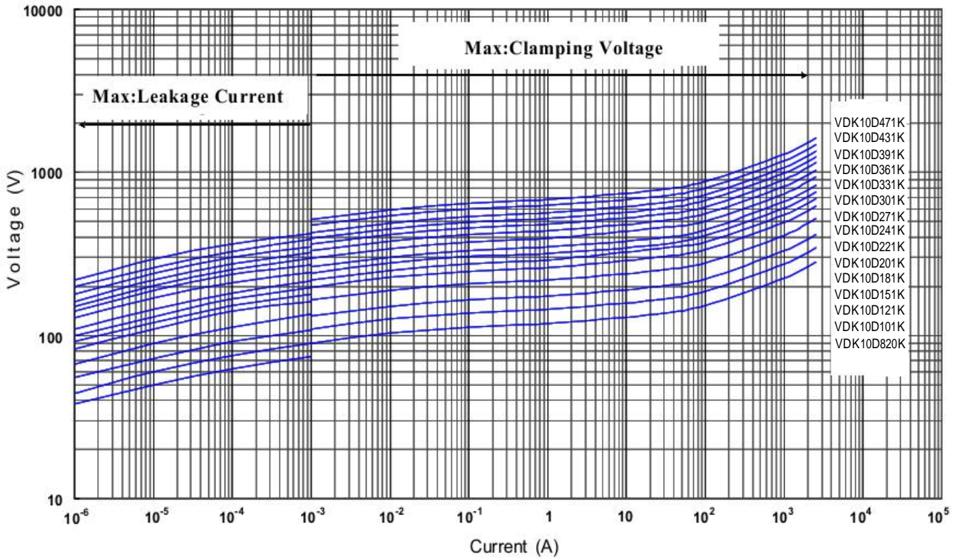
V-I Curve (VDK-10D820K to VDK-10D471K)
