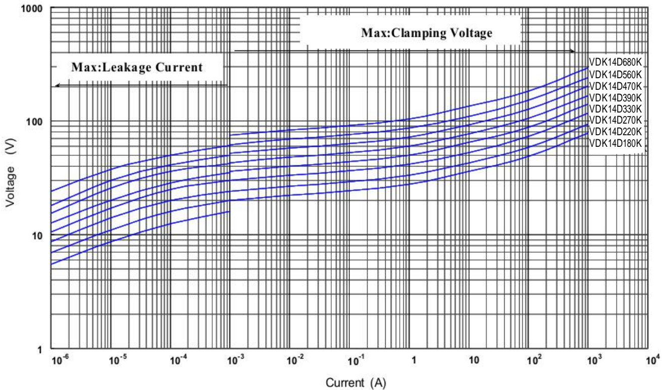
V-I Curve (VDK-14D180K to VDK-14D680K)
