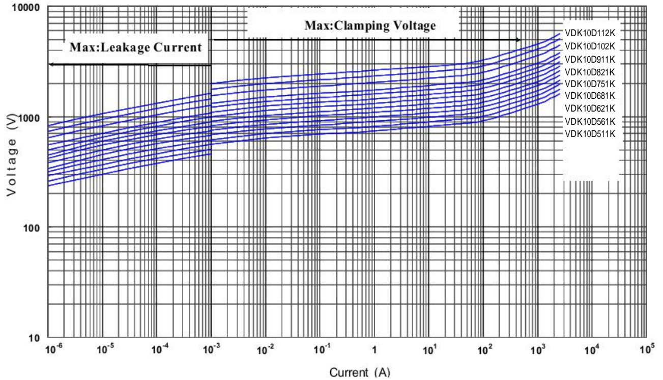
V-I Curve (VDK-10D511K to VDK-10D112K)
