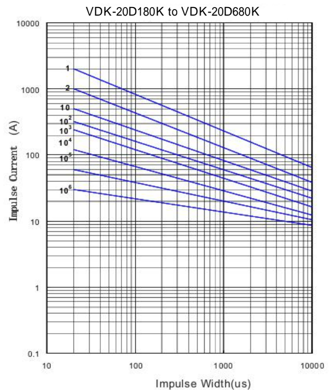
VDK-20D Series
