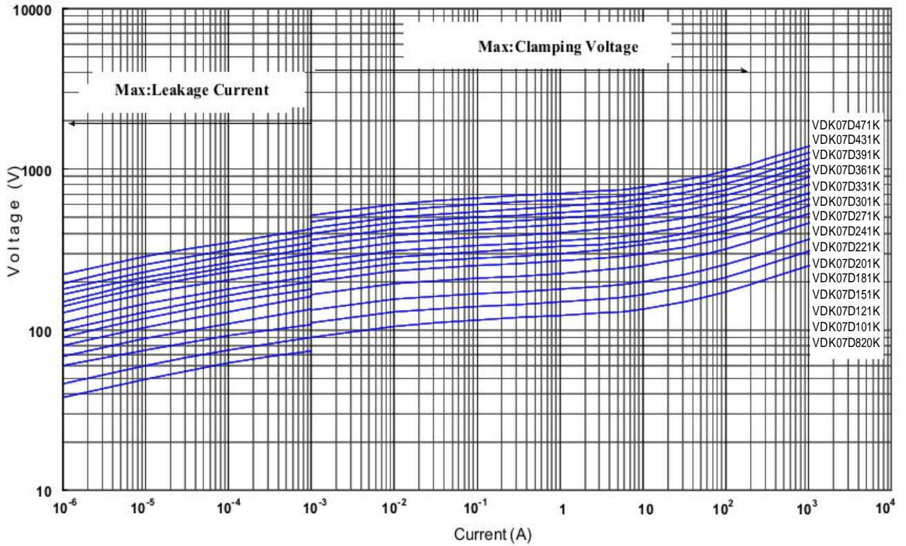
V-I Curve (VDK-07D820K to VDK-07D471K)
