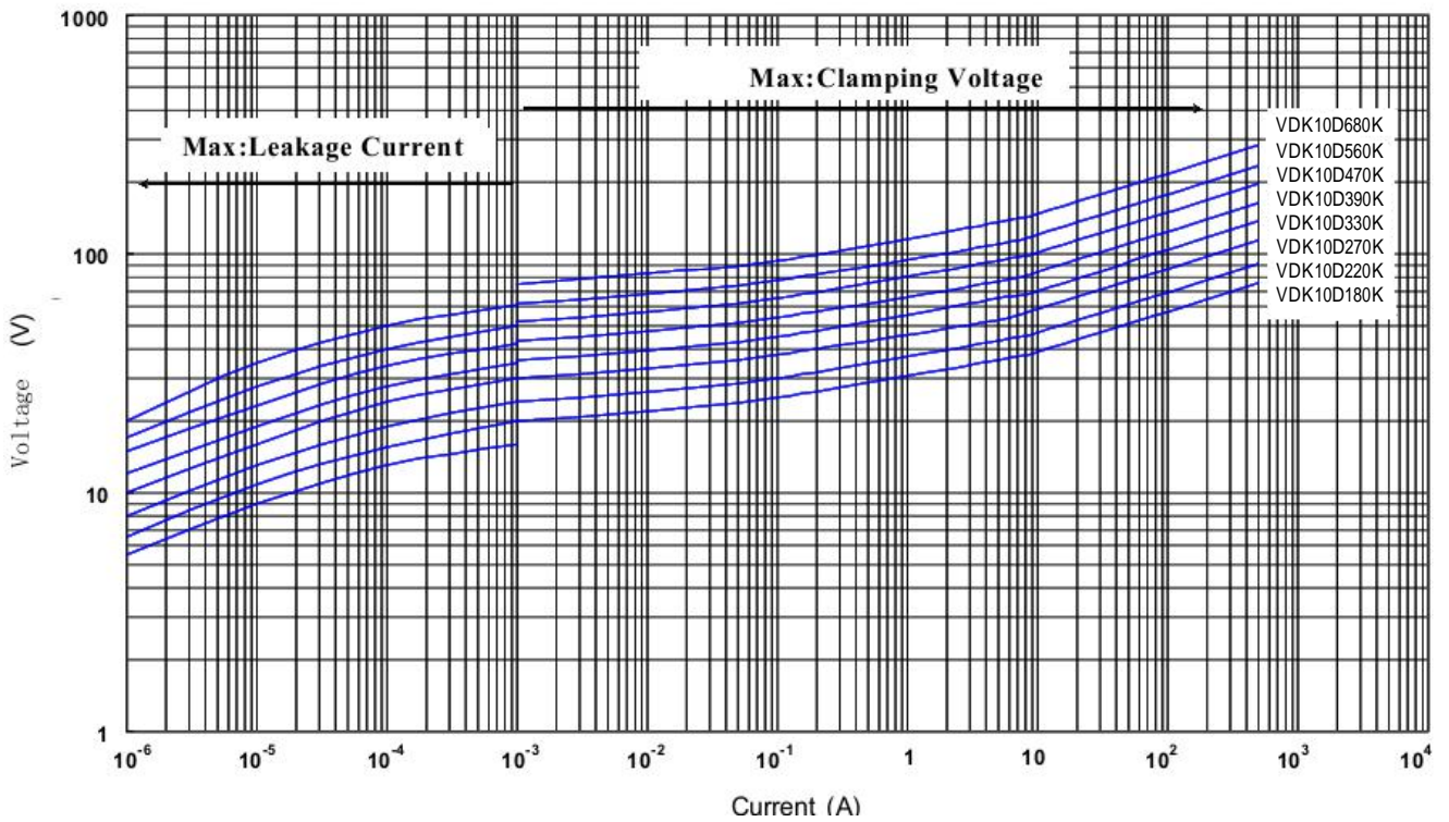
V-I Curve (VDK-10D180K to VDK-10D680K)
