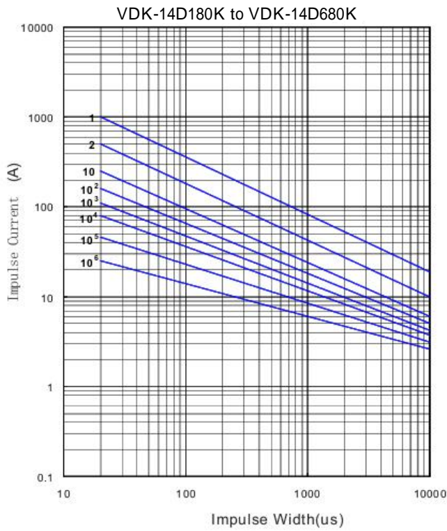
VDK-14D Series
