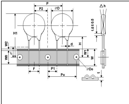
(图 1: Straight Leads 05\07D\10D)
