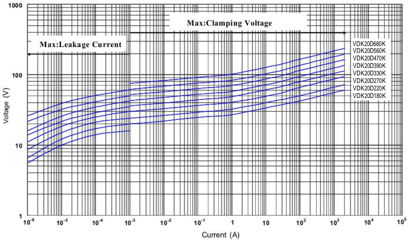
V-I Curve (VDK-20D180K to VDK-20D680K)
