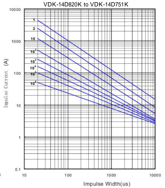
VDK-14D Series
