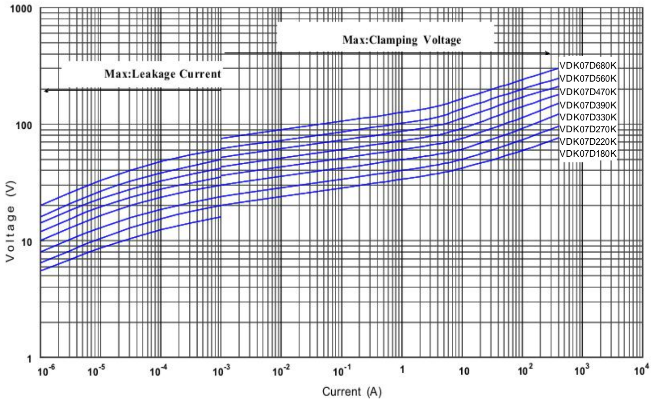
V-I Curve (VDK-07D180K to VDK-07D680K)
