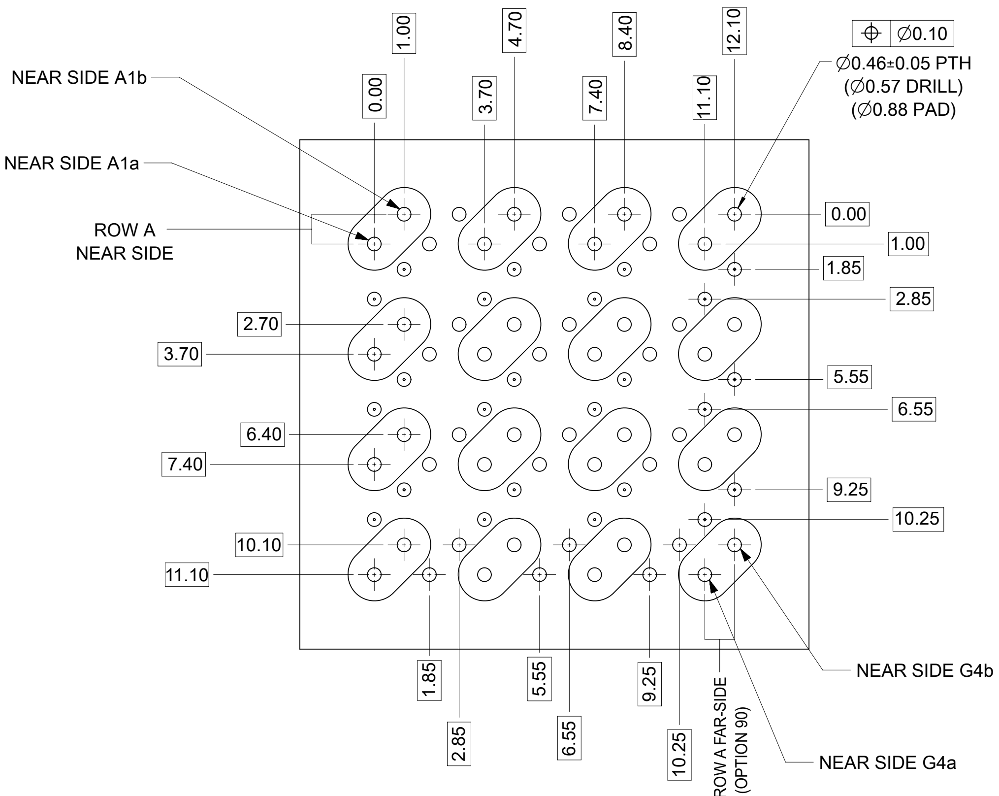
Orthorogonal PCB Layout
