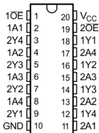
Figure 5-1. DB, DGV, DW, NS, PW Package, 20-Pin SSOP, TVSOP, SOIC, SO, TSSOP (Top View)
