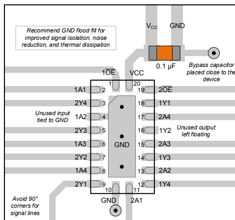
Figure 11-1. Layout Example for the SN74LV244A in the RKS Package
