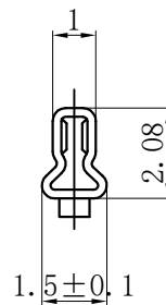
SECTION C-C
