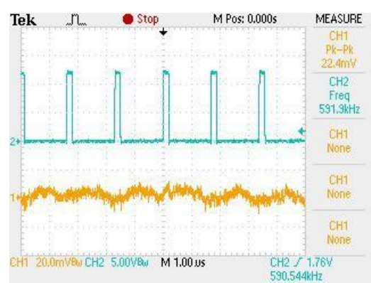
STEADY STATE OPERATION (VIN=12V,VOUT=1.2V,IOUT=1000mA)
