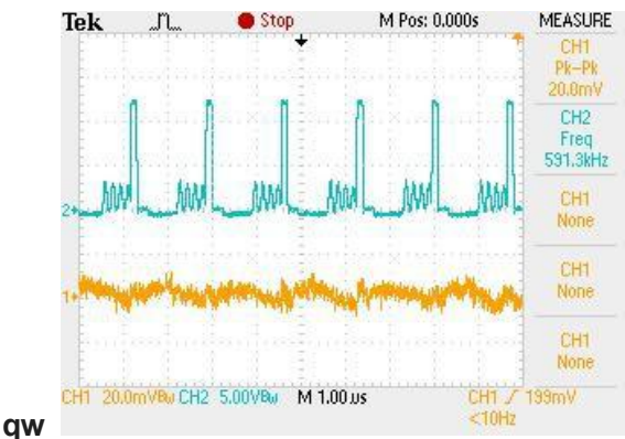
STEADY STATE OPERATION (VIN=12V,VOUT=1.2V,IOUT=100mA)
