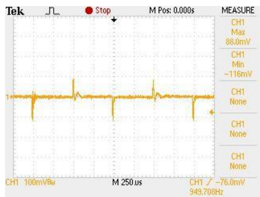
LOAD TRANSIENT RESPONSE (VIN=12V,VOUT=1.2V,IOUT=100-1000mA,1A/μs)
