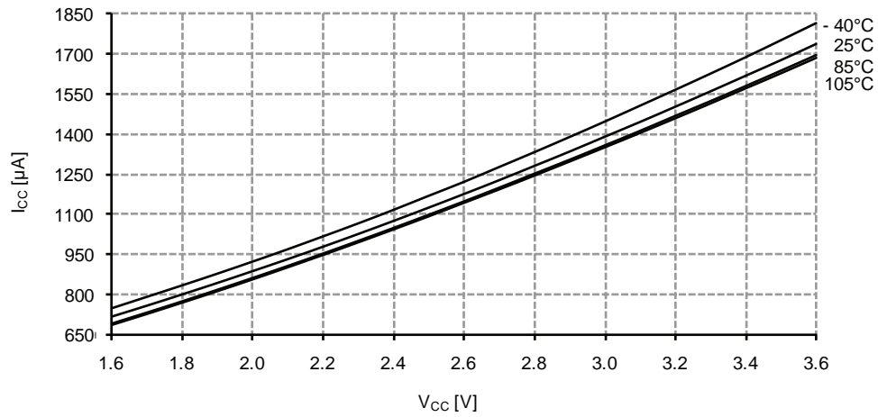
Figure 33-172. Idle Mode Current vs. V_{CC}
