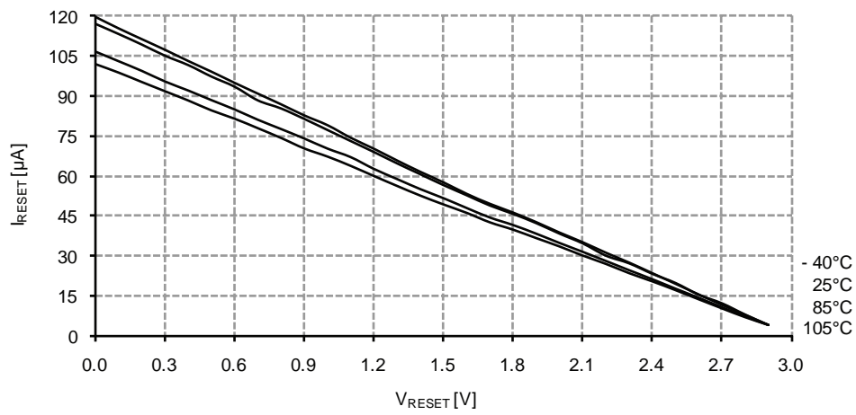
Figure 33-222. Reset Pin Pull-up Resistor Current vs. Reset Pin Voltage
