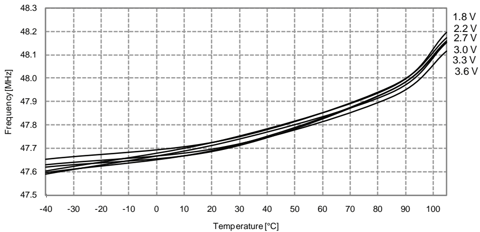
Figure 33-322. 48MHz Internal Oscillator Frequency vs. Temperature DPLL enabled, from the 32.768kHz internal oscillator
