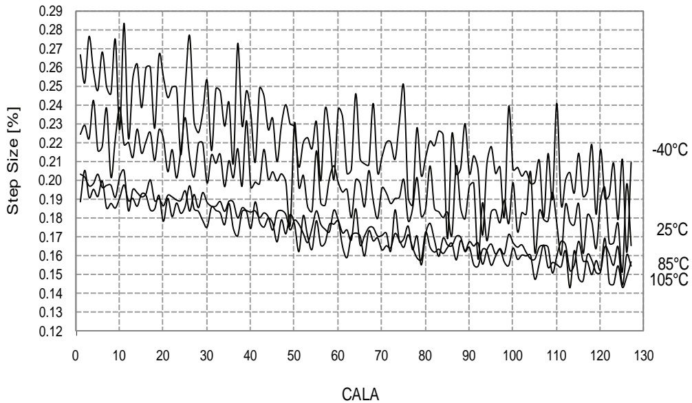
Figure 33-70. 2MHz Internal Oscillator CALA Calibration Step Size
