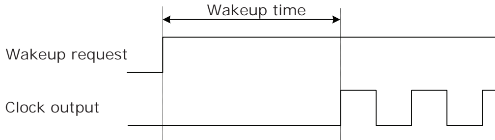
Figure 32-2. Wake-up Time Definition
