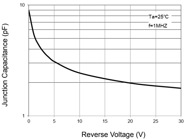
Fig 4. Junction Capacitance
