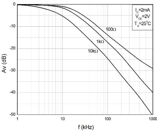
Fig.11 Frequency Response
