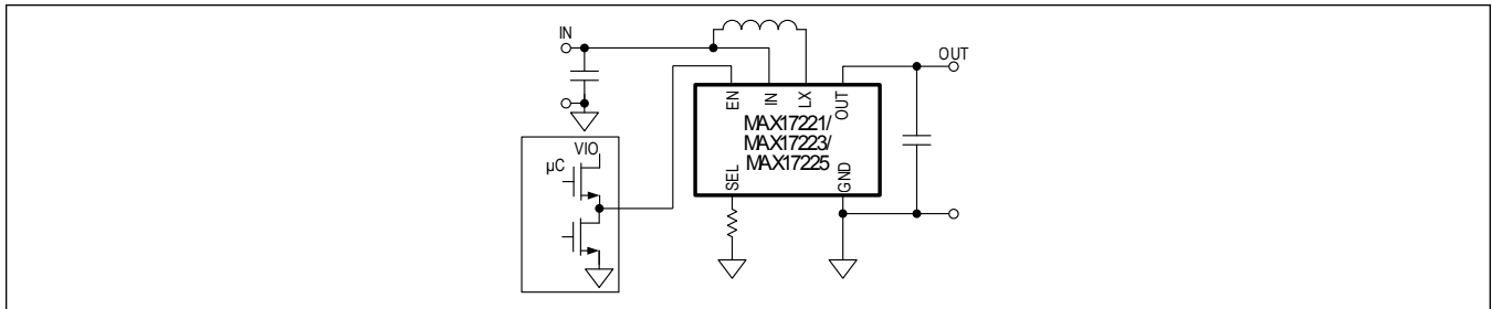
Figure 2. Only the MAX17221/MAX17223/MAX17225 EN Pin Can Be Driven by a Push-Pull Microcontroller GPIO.
