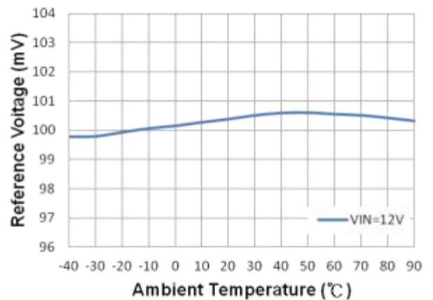
Figure 17. Reference Voltage vs. Temperature ( I_{OUT}=0.5A , 2S2P LED)
