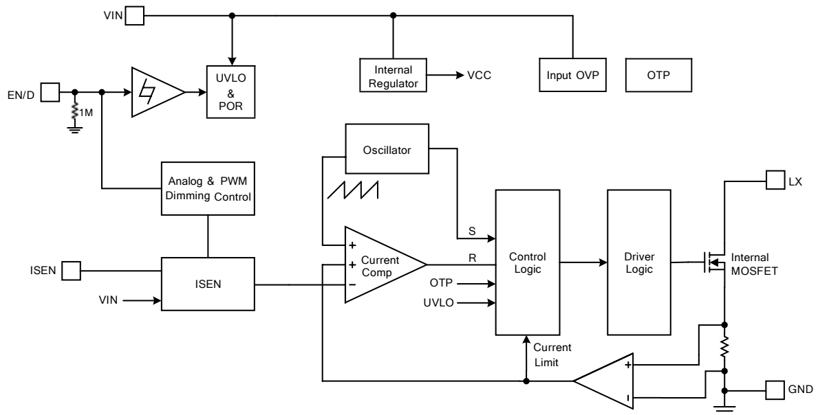
Figure 5. Block Diagram of FR9703
