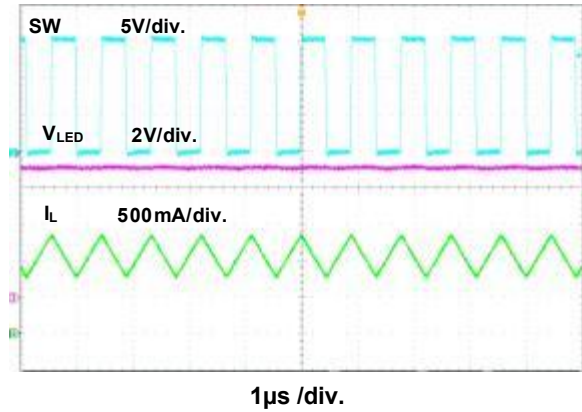
Figure 7. Switching Waveform
