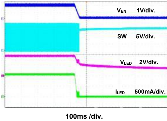
Figure 12. Power Off through V_{EN} Waveform
