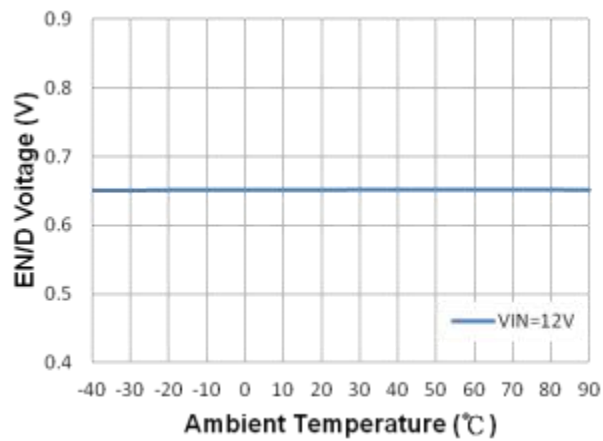
Figure 18. EN/D Voltage vs. Temperature ( I_{OUT}=0.5A , 2S2P LED)
