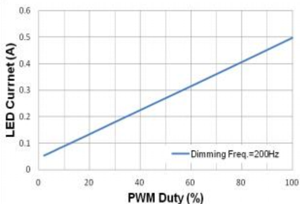
Figure 20. Digital Dimming: I_{LED} vs. PWM Duty ( V_{IN}=12V , 3S2P LED)
