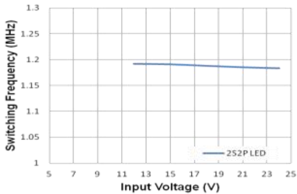
Figure 14. Frequency vs. Input Voltage ( I_{OUT}=0.5A )
