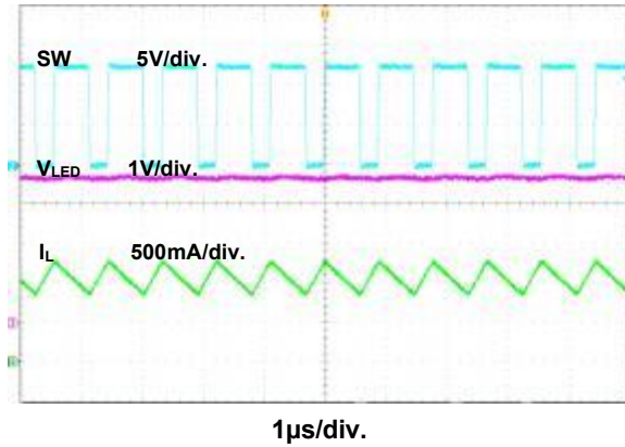
Figure 6. Switching Waveform
