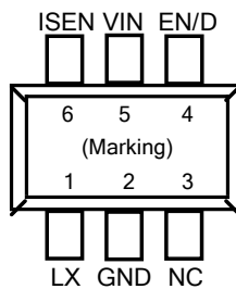
Figure 1. Pin Assignments of FR9703
