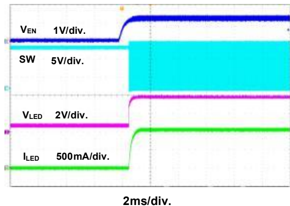
Figure 11. Power On through EN Waveform
