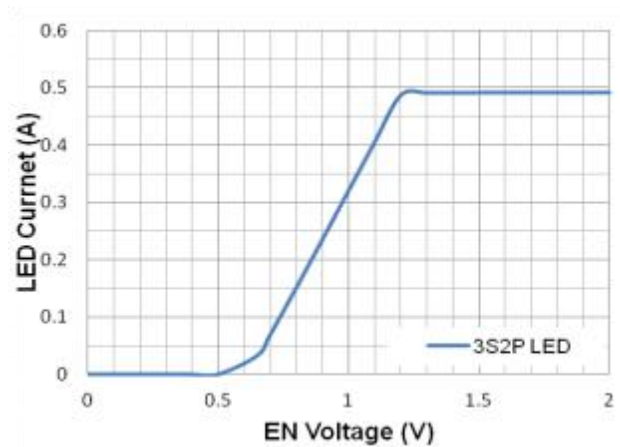
Figure 19. Analog Dimming: I_{LED} vs. EN Voltage ( V_{IN}=12V )
