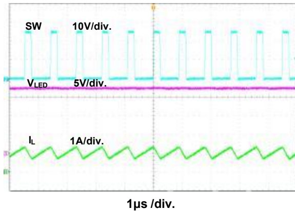
Figure 8. Switching Waveform
