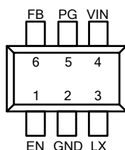
Figure 1. Pin Assignment of FP6397
