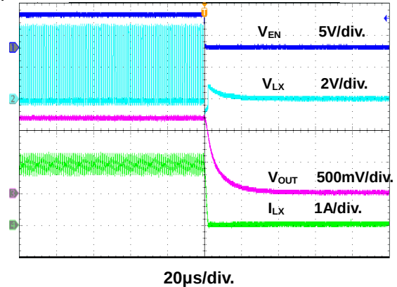
Figure 15. Power Off through EN Waveform
