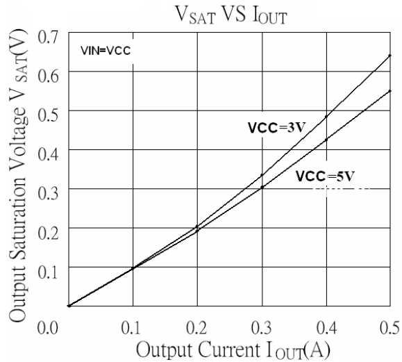
Figure 4a. V_{SAT} vs. I_{OUT}
