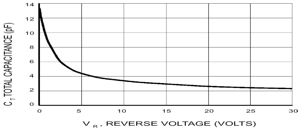
Fig.3 C_T — V_R
