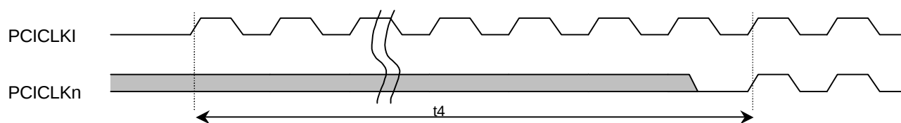
Figure 7-4. PCI Clock Acquisition Timing
