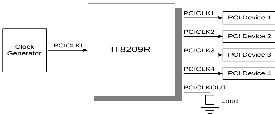
Figure 3-2. Clock Buffer Scheme
