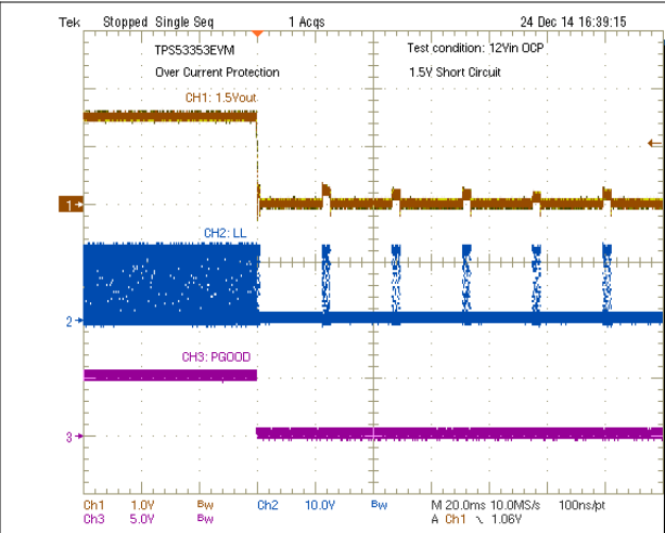
Figure 8-12. Output Short-Circuit Protection
