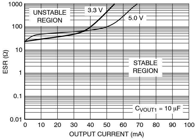
Figure 26. V_{OUT1} Output Capacitor ESR (10 \mu\text{F} )
